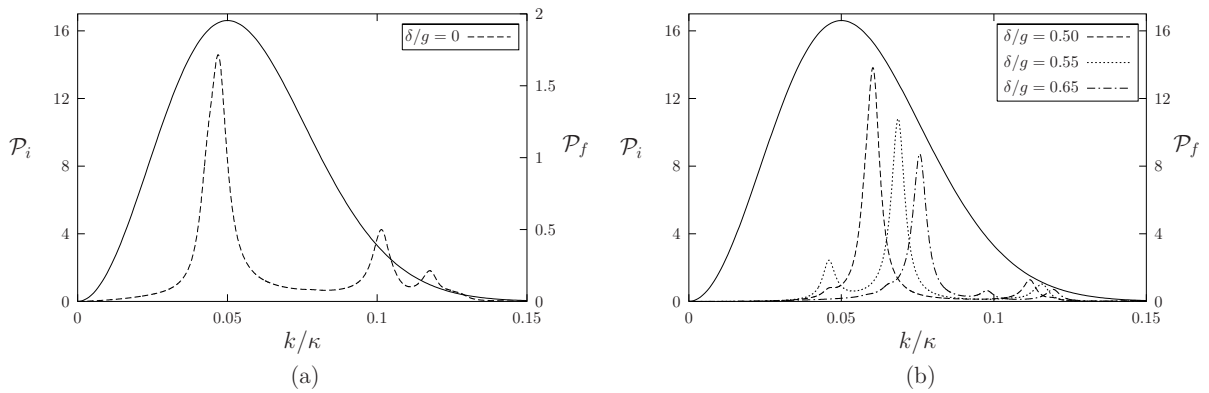
FIG. 8 – Initial (plain curve) and final (dashed curves) velocity distributions (a) at resonance and (b) for various detuning values.
